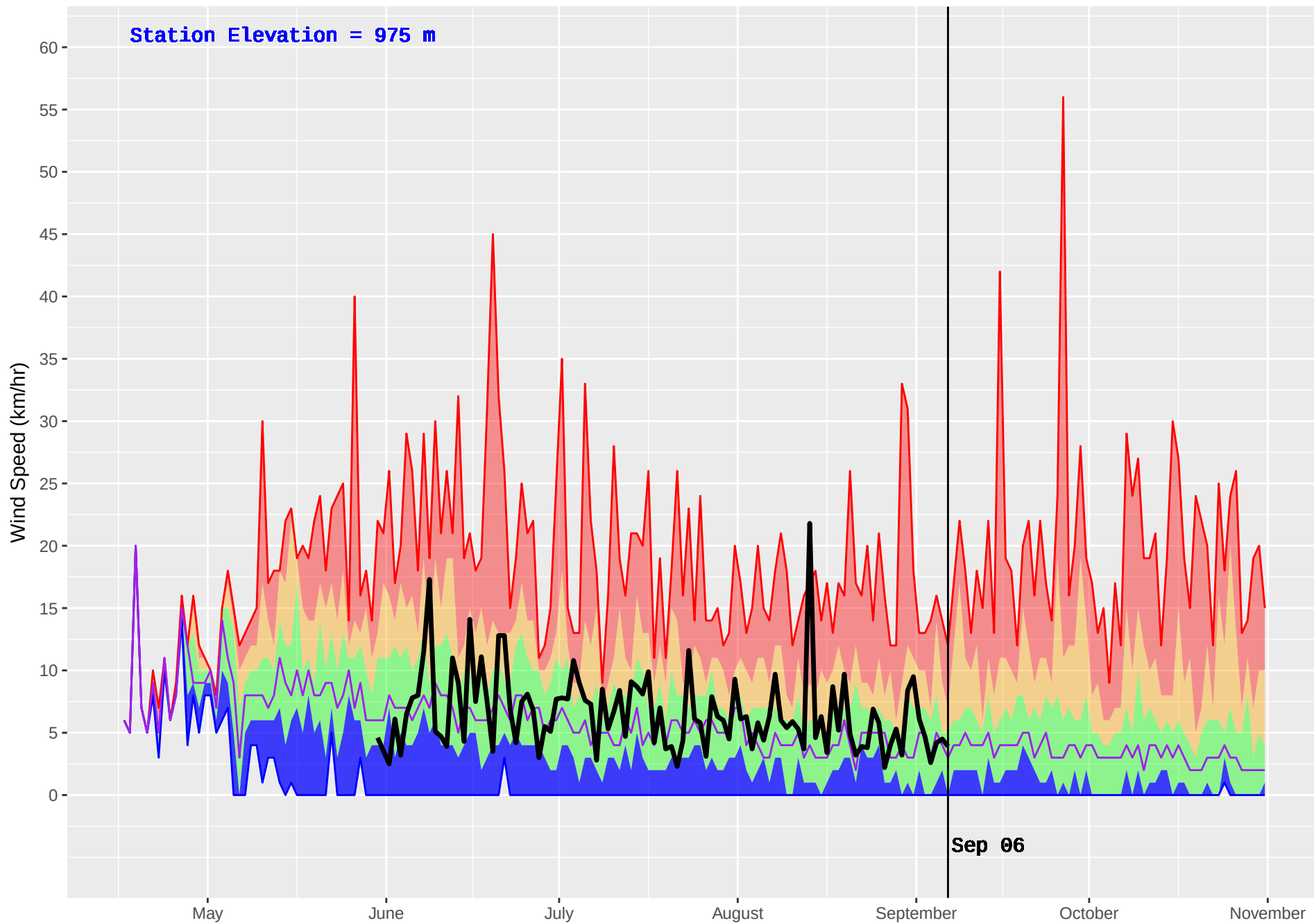
MCGREGOR 2 (192) : Historical (1986–2016) and Current (2017) Noon Wind Speed
