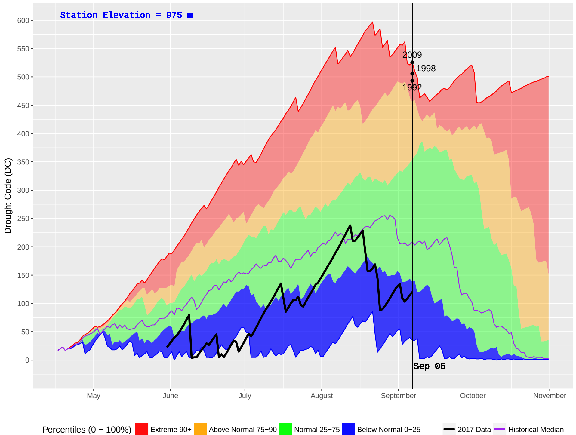
MCGREGOR 2 (192) : Historical (1986–2016) and Current (2017) Noon Drought Code (DC)
